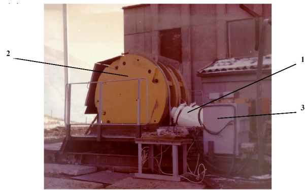
Fig. 2. Pulsed MHD generator installed at Bishkek geophysical proving ground (Kyrgysia, Northern Tien-Shan); 1 – solid propellant plasma generators; 2 – magnet system; 3 – electric switching equipment
